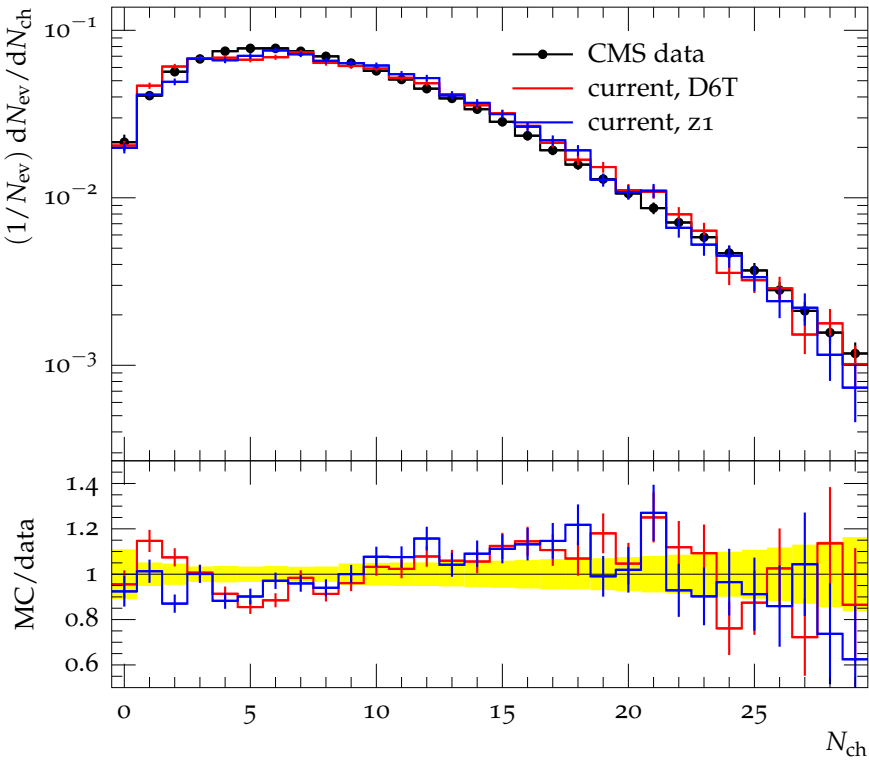
Distribution N_{\text{ch}} at 7 TeV, \text{max } p_{\text{T}} > 3 \text{ GeV}/c
