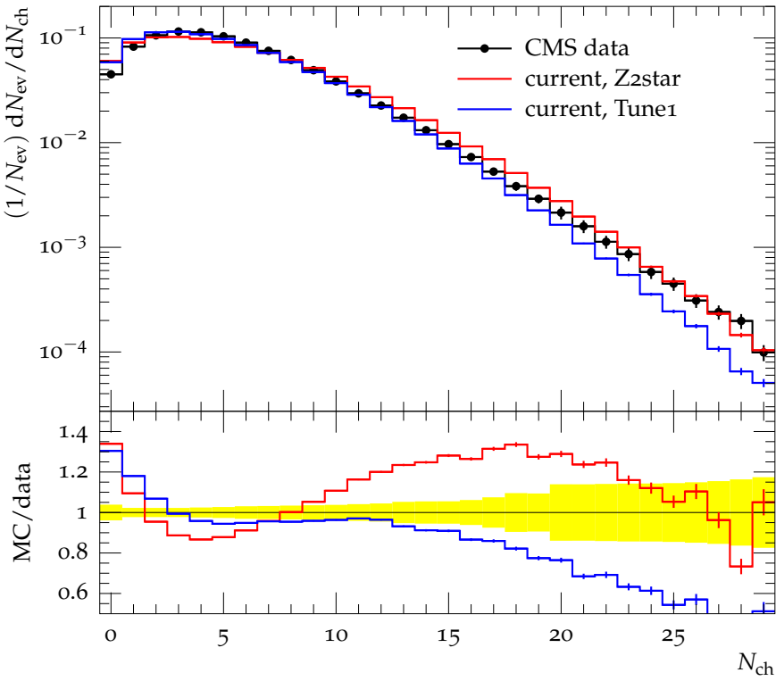
Distribution N_{\text{ch}} at 7 TeV, \max p_T > 20 \text{ GeV}/c
