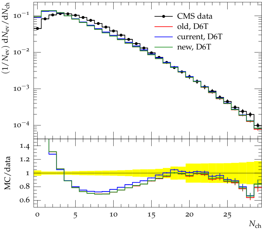
Distribution N_{\text{ch}} at 7 TeV, max p_{\text{T}} > 20 GeV/c
