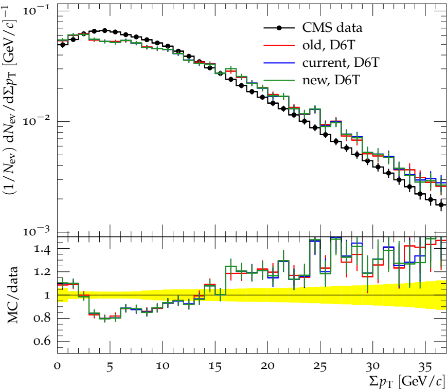
Distribution \Sigma p_T at 7 TeV, max p_T > 3 GeV/c
