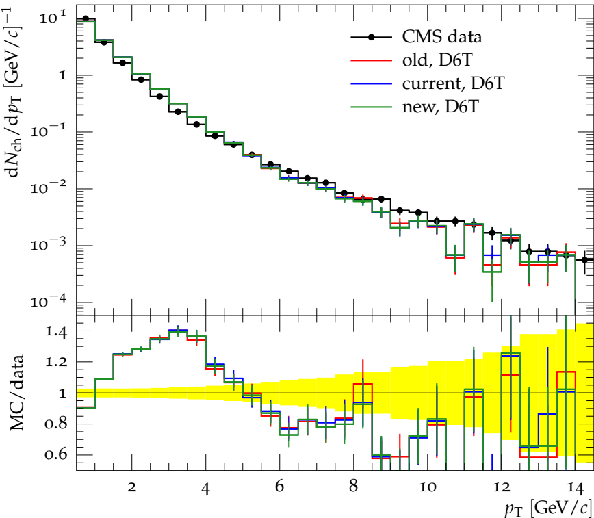
Distribution p_T at 7 TeV, max p_T > 3 GeV/c
