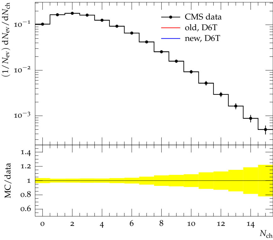
Distribution N_{\text{ch}} at 0.9 TeV, max p_T > 3 GeV/c
