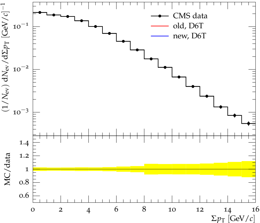
Distribution \Sigma p_T at 0.9 TeV, max p_T > 3 GeV/c
