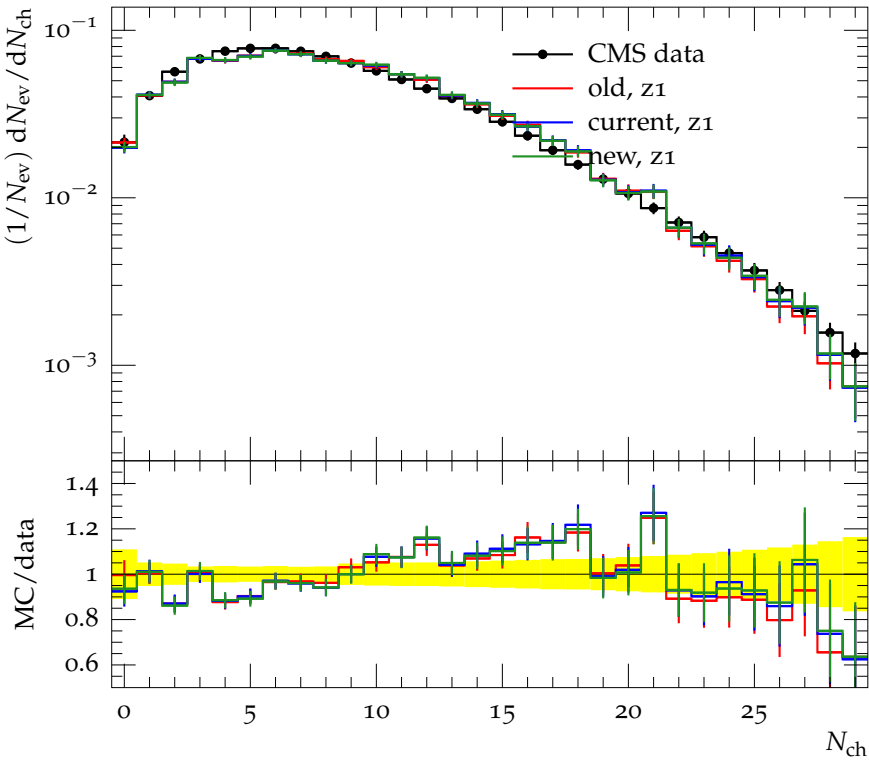
Distribution N_{\text{ch}} at 7 TeV, \max p_T > 3 \text{ GeV}/c
