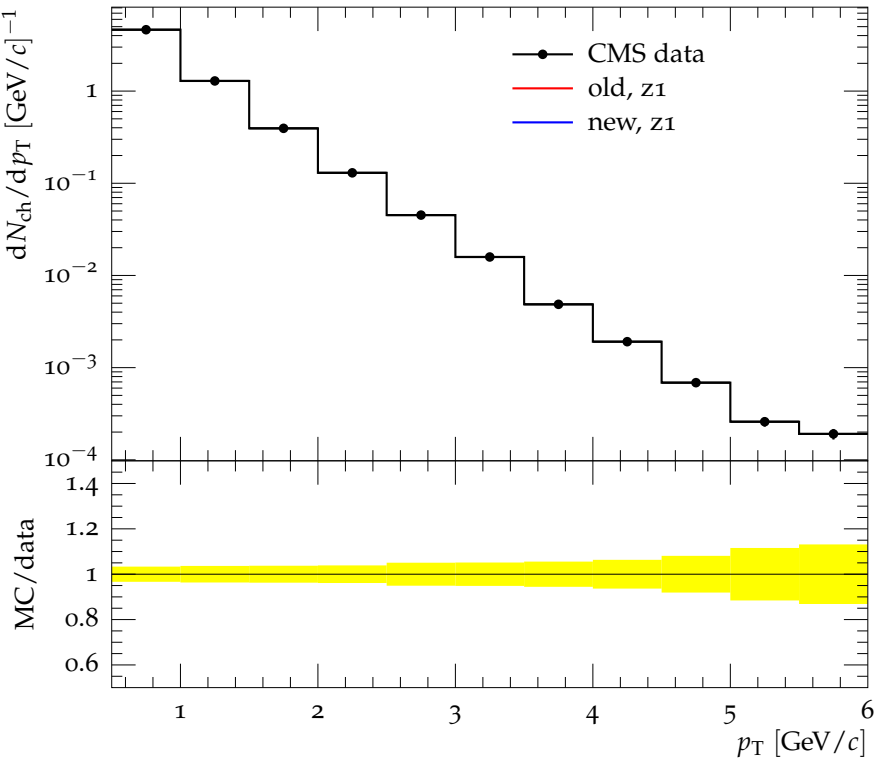
Distribution p_T at 0.9 TeV, max p_T > 3 \text{ GeV}/c
