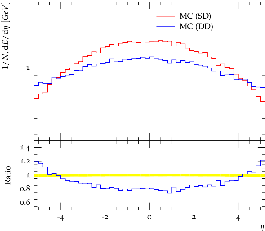
Energy flow as a function of rapidity
