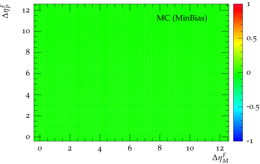
Large Rapidity Gap 2D Histogram
