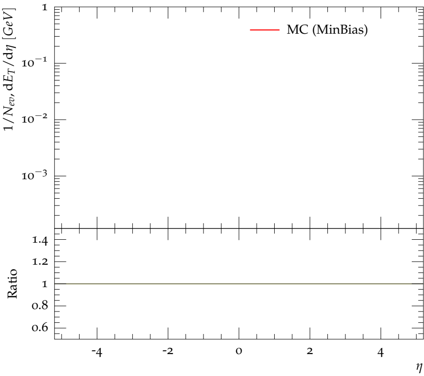
Transverse energy flow as a function of rapidity
