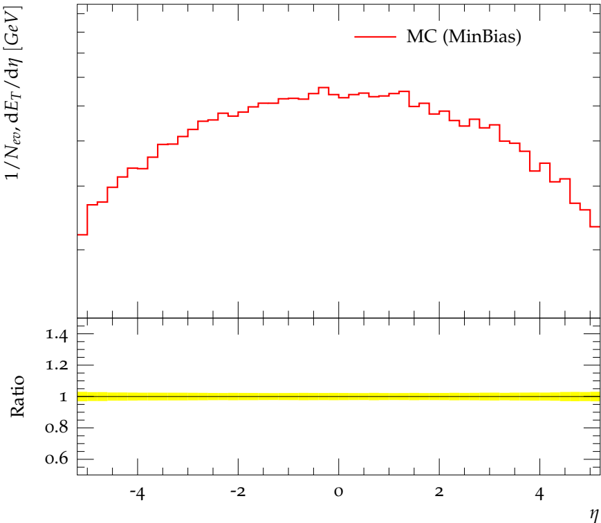
Transverse energy flow as a function of rapidity
