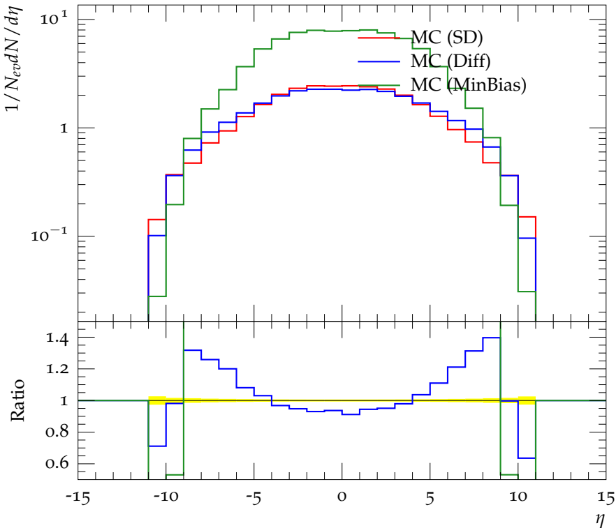
\eta Distribution of Final State Particles
