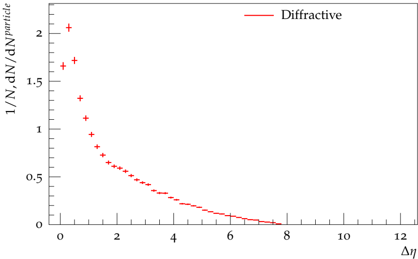
Charged Particle Multiplicity vs Gap Size
