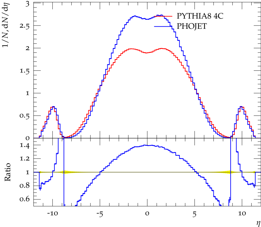
\eta distribution of final state particles
