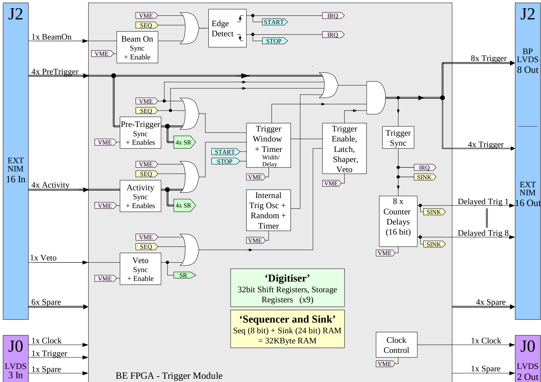
Trigger Logic Block Diagram (v3 - 25/6/2003)
