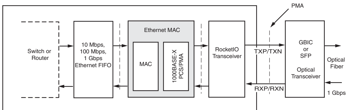
Figure 3: Typical 1000BASE-X Application
